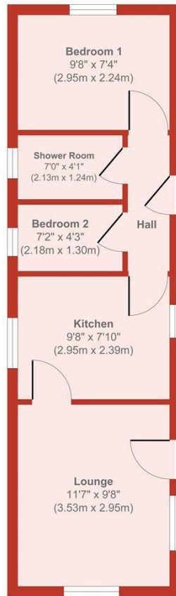
Floor Plan
